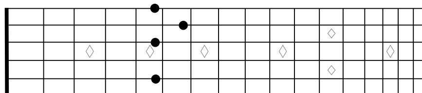
Dm7/A
